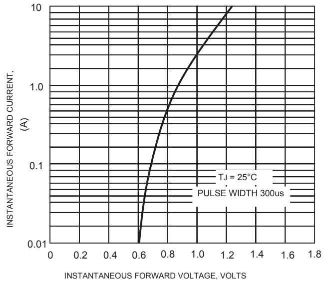
FIG.4-TYPICAL FORWARD CHARACTERISTICS
